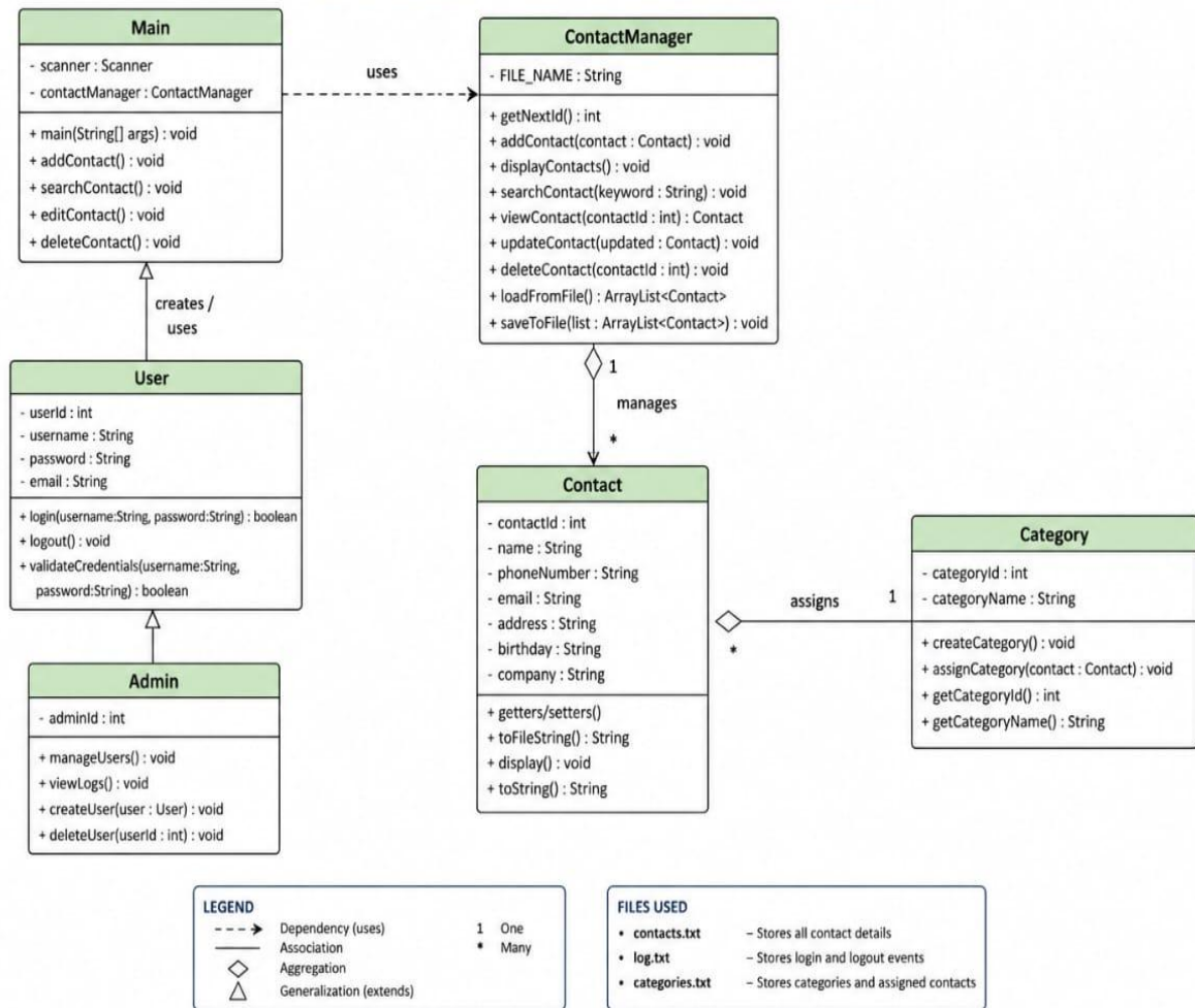
CLASS DIAGRAM – CONTACT MANAGEMENT SYSTEM
